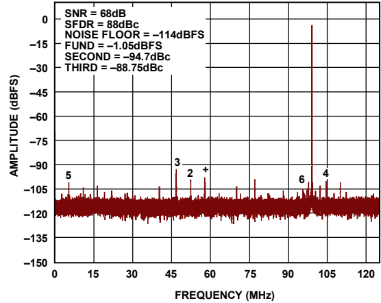
Figure 56. Measured Single-Tone Performance of the Circuit Shown in Figure 54 for a 100 MHz Input Signal
