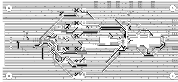
Figure 63. Bottom Layer
