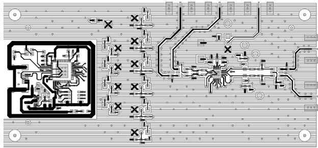
Figure 62. Top Layer
